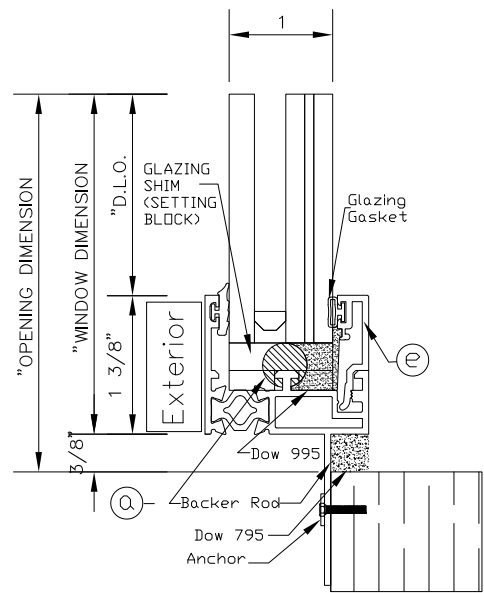
D SILL Frame Depth: 1.625
