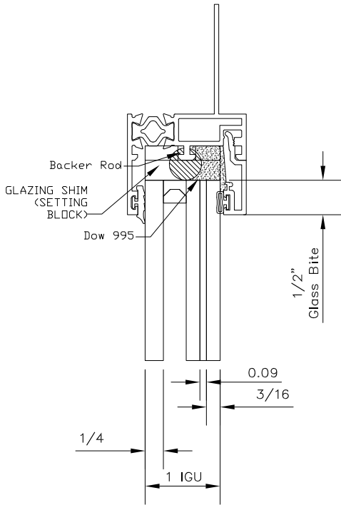
I. FIXED WINDOW GLAZING DETAILS
