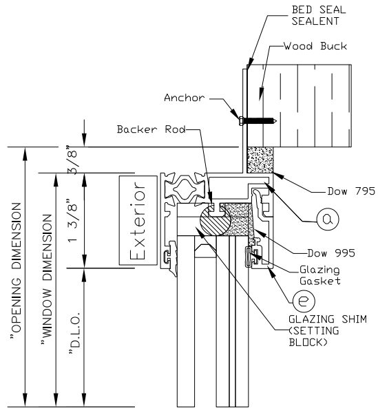
A HEAD Frame Depth: 1.625
